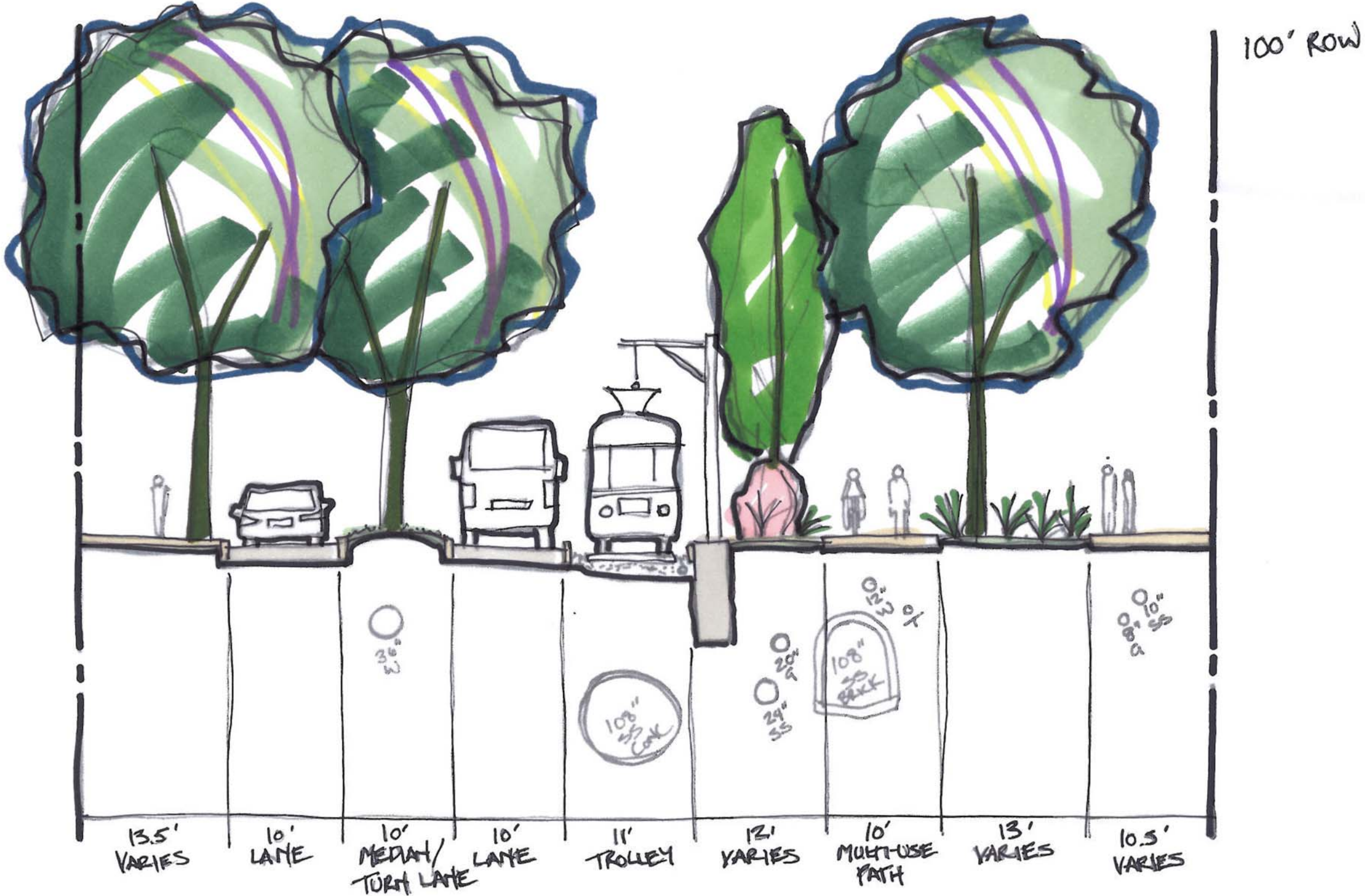
Section AA (Looking North)
